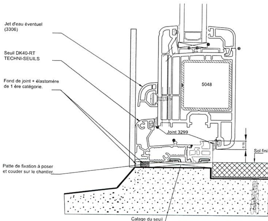
5048 seuil TECHNI-SEUILS DK40-RT
